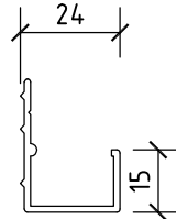
Corner Profiles 135°
