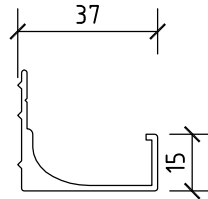
Corner Profiles
