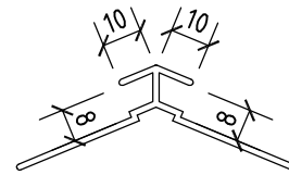
Corner Profiles 135°
