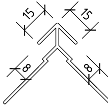
Corner Profiles
